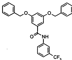
Compound # 8
